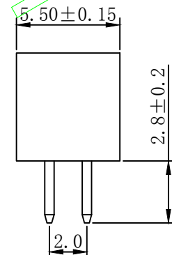
Plastic Base
